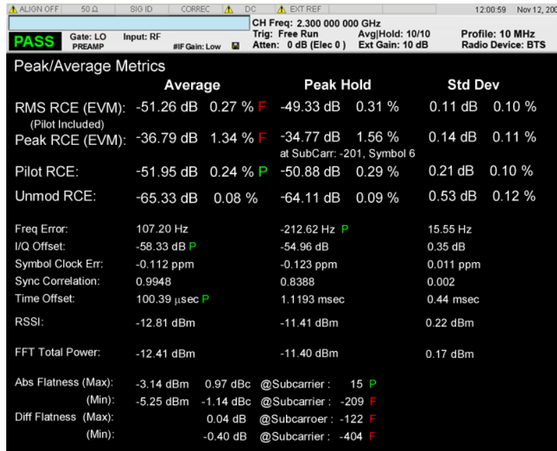
Figure 6-9 Peak/Average Metrics Table
