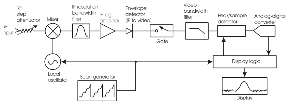
Figure 6-15 Gated Video Signal Analyzer Block Diagram
