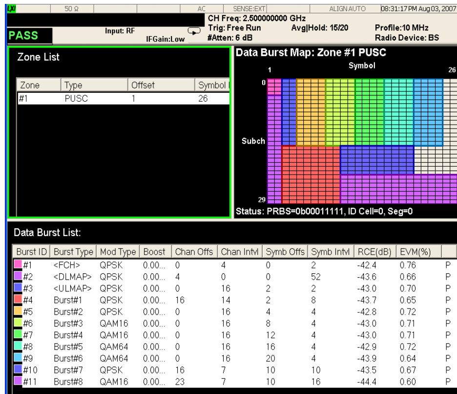
Figure 3-22 Modulation Accuracy Measurement Result - Zone & Data Burst Info View
