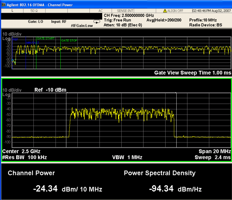
Figure 3-2 Channel Power Measurement Result - Gate View w/Gate in Data Burst
