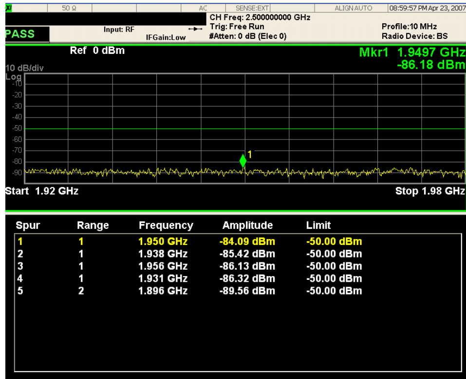
Spurious Emissions Measurement - Default Result
