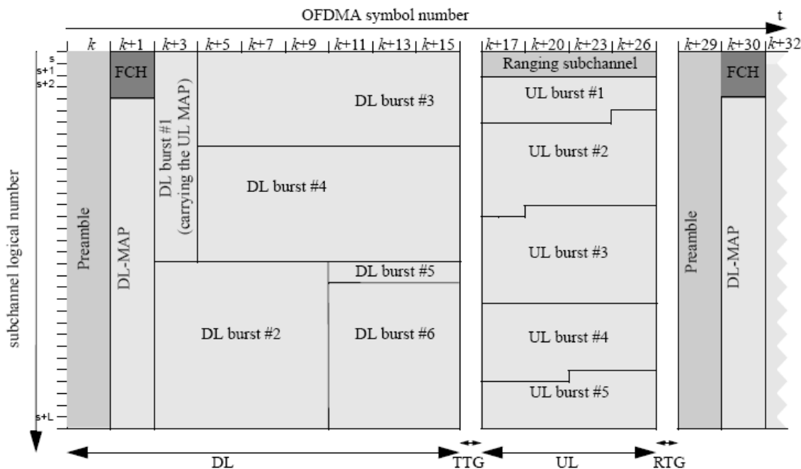
Figure 6-33 OFDMA Frame Structure
