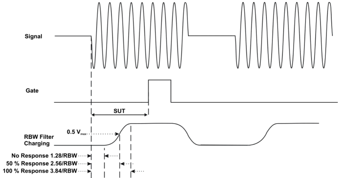
Figure 6-27 Resolution Bandwidth Filter Charge-Up Effects
