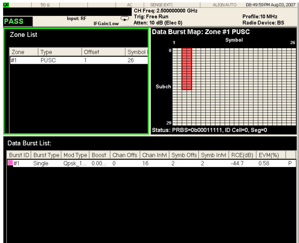
Figure 3-29 Modulation Accuracy Measurement Result - Zone & Data Burst Info (Single Burst) View
