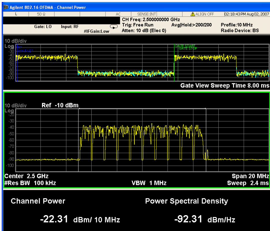
Figure 3-3 Channel Power Measurement Result - Gate View w/Gate in Preamble of Second Burst
