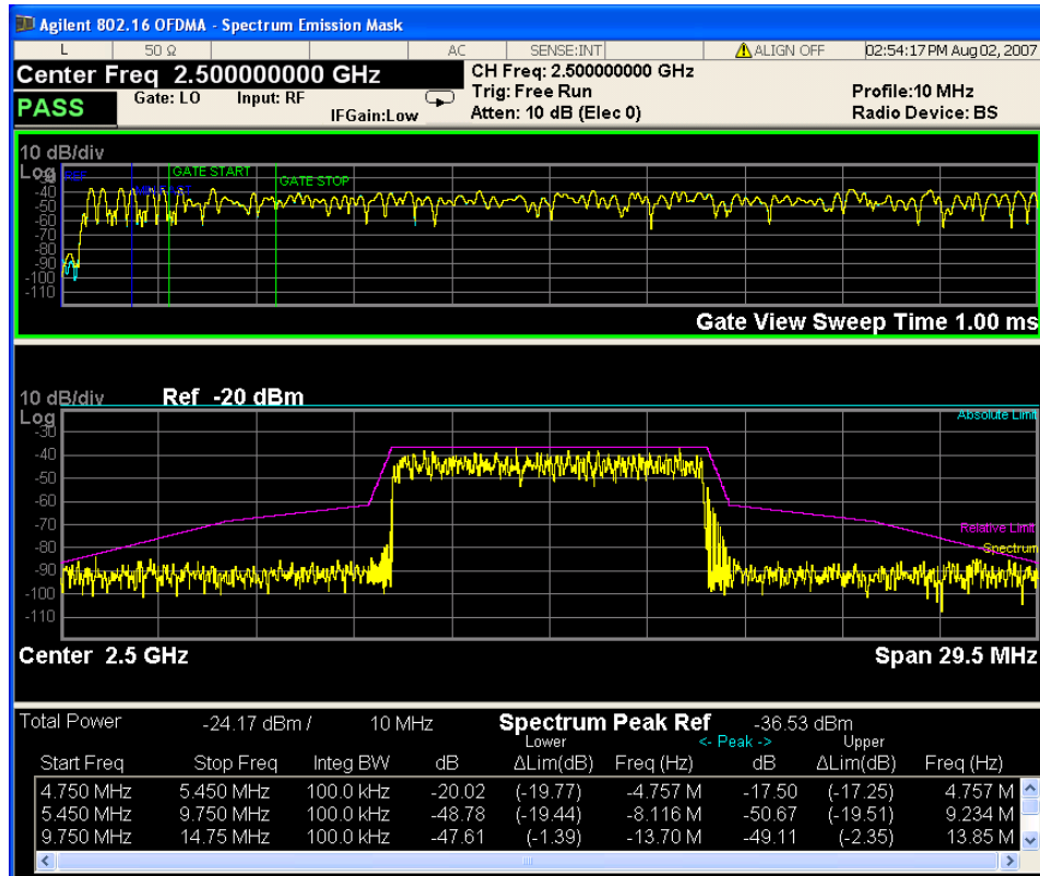
Figure 3-8 Spectrum Emission Mask (Total Pwr) Measurement Result - Relative Pwr Ref View
