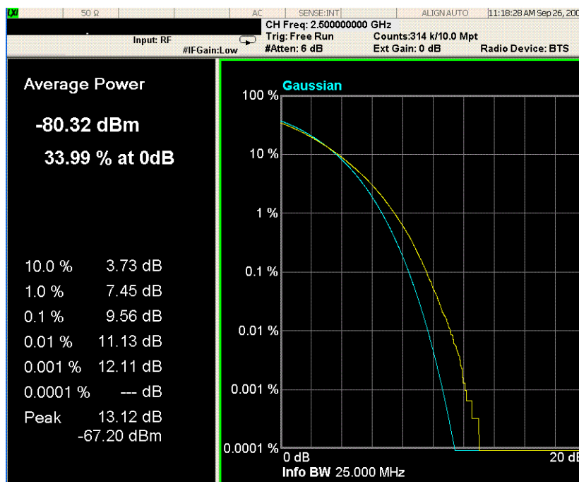
Figure 3-31 Power Statistics CCDF Result
