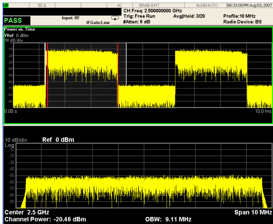
Figure 3-27 Modulation Analysis Measurement Result - Power vs. Time and Spectrum View
