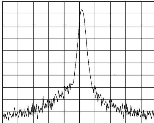
Figure 6-13 Time-Gated Spectrum of Radio 2
