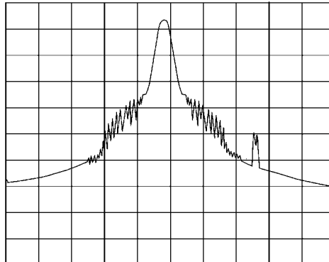
Figure 6-12 Time-Gated Spectrum of Radio 1
