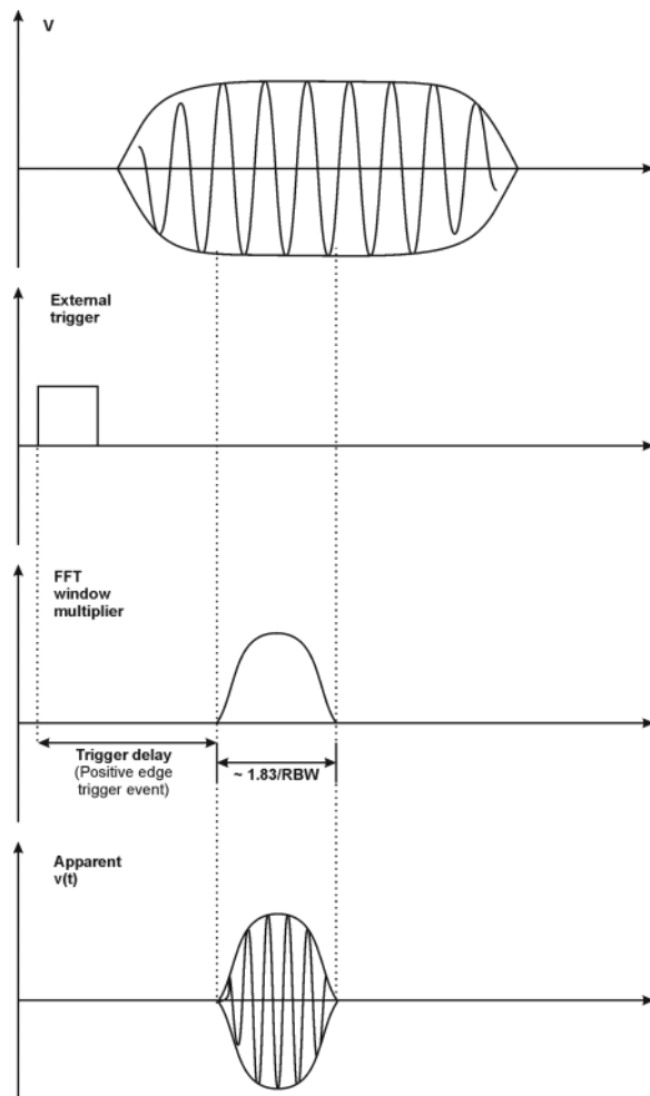
Figure 6-17 Gated FFT Timing Diagram
