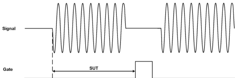
Figure 6-26 Setup Time for Interpulse Measurement
