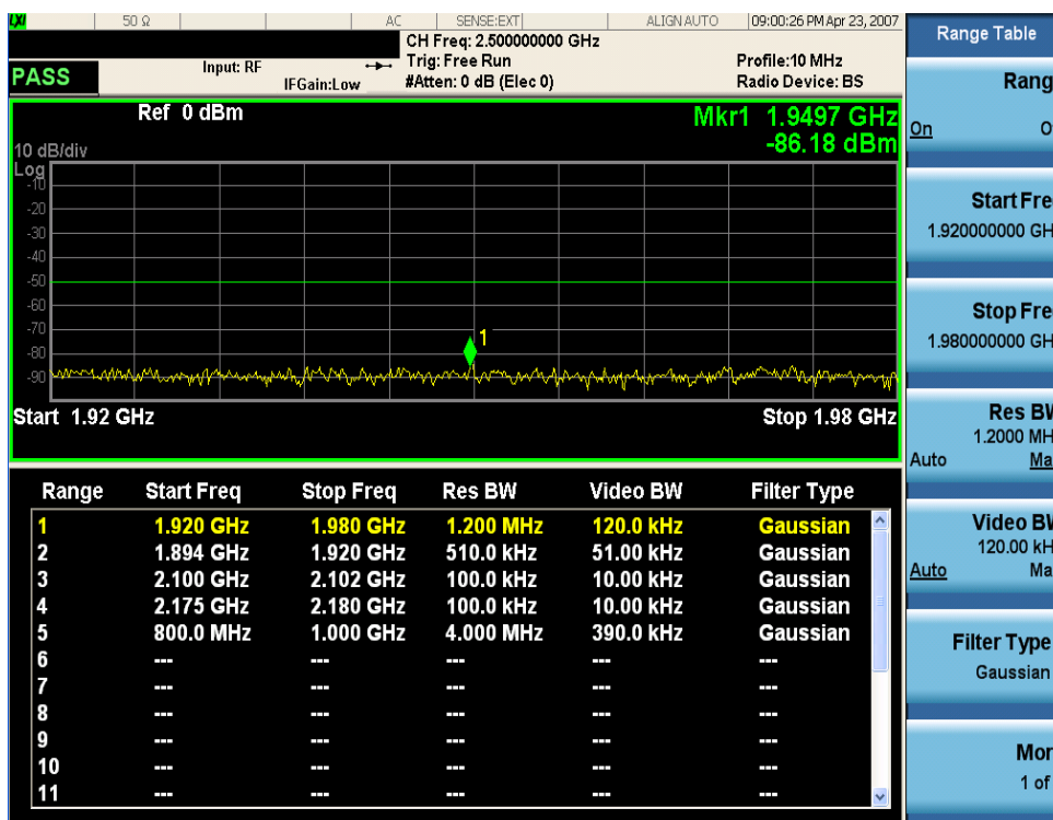
Figure 3-13 Spurious Emissions Measurement - Range Table View 1
